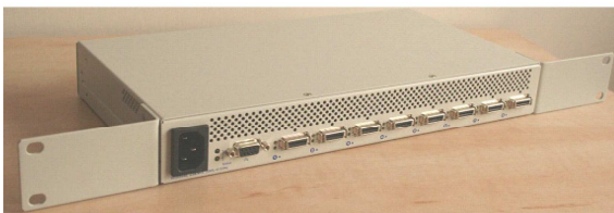
Figure 6: View of Rack Adapter Assembled on Rear Panel Sides
